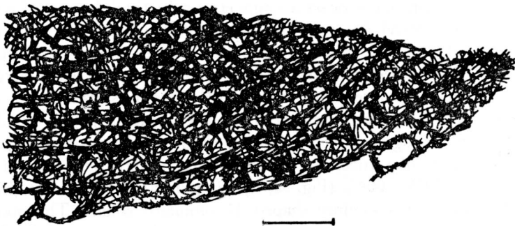
FIGURE 6. Xestospongia rosariensis , longitudinal section through apex of a tube showing radiate-accretive structure (scale = 1 cm).
