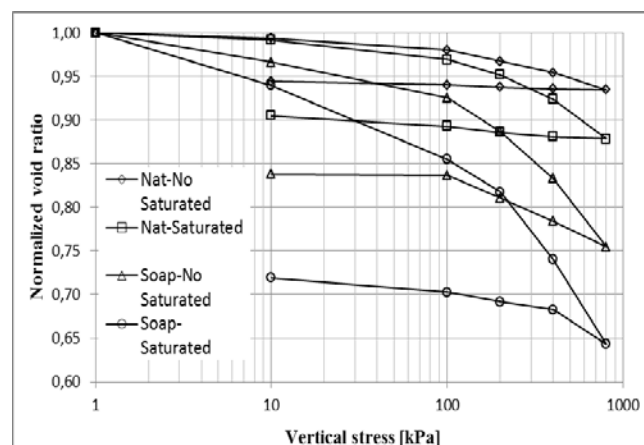
Figure 5. Result of the double-edometric test Source: The authors
