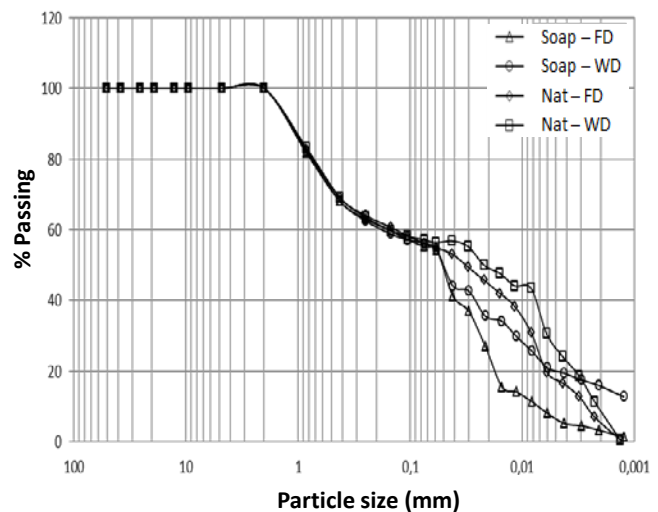
Figure 1. Granulometric curve of the soil Source: The authors
