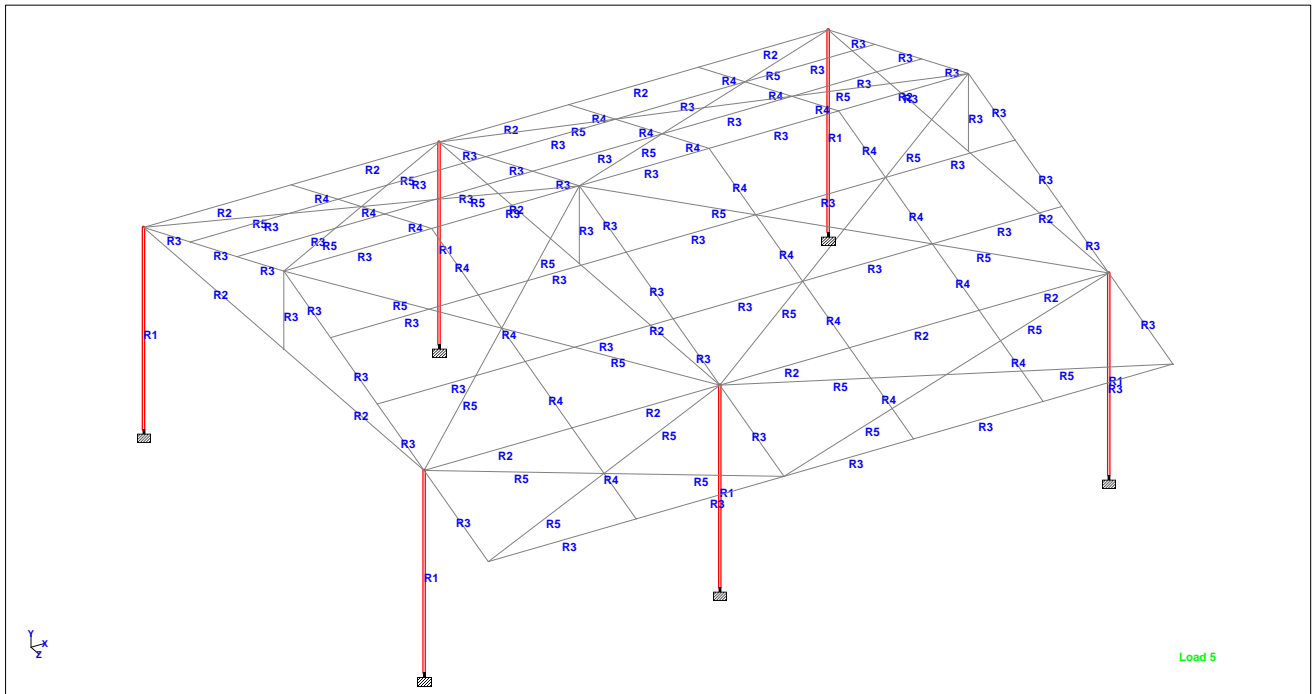
COLUMNAS PERFILES TUBULARES 160X160X6 MM.
