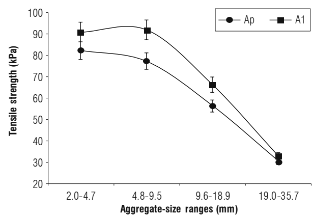
FIGURE 2. Distribution of the TS per horizon for the different aggregate-size ranges (confidence interval 95%) for soils cultivated with sugar cane (Colombia).
